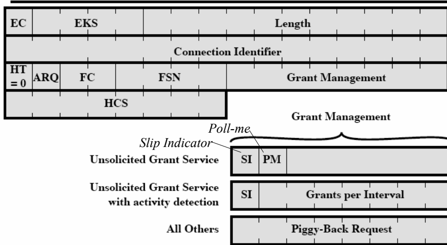
(b) Generic uplink header
