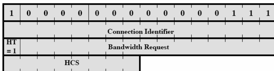
(c) Bandwidth request header
